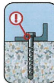
Installation was successful when the head of the anchor is fully supported on the fixture and it is not damaged
